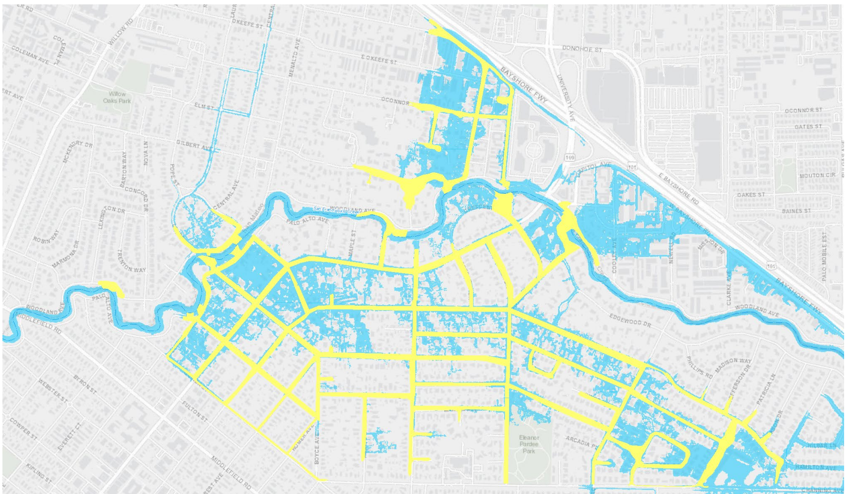
FIGURE B-2: Revised Model NYE Flooding (Blue), NYE Approximate Observed Flooding (Yellow)
